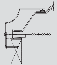
Curb Mount
